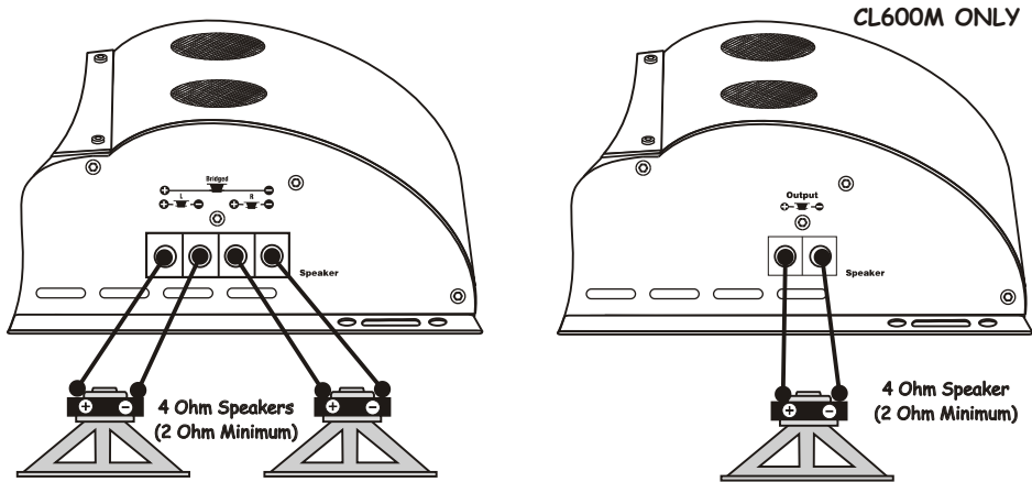
TWO CHANNEL SPEAKER CONNECTIONS
